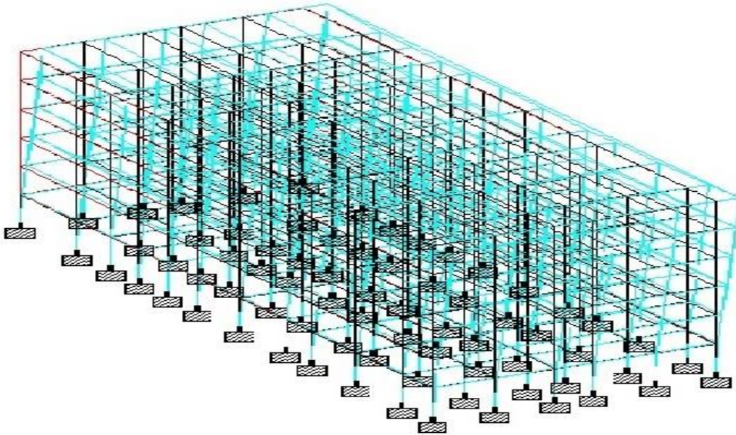
Fig 10 Deflection diagram
