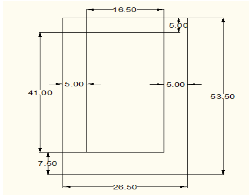
Fig.2 plinth area
