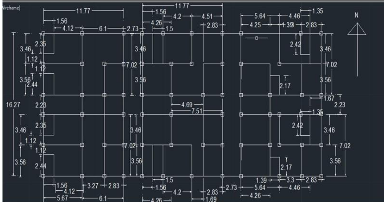
Fig 4 structural plan
